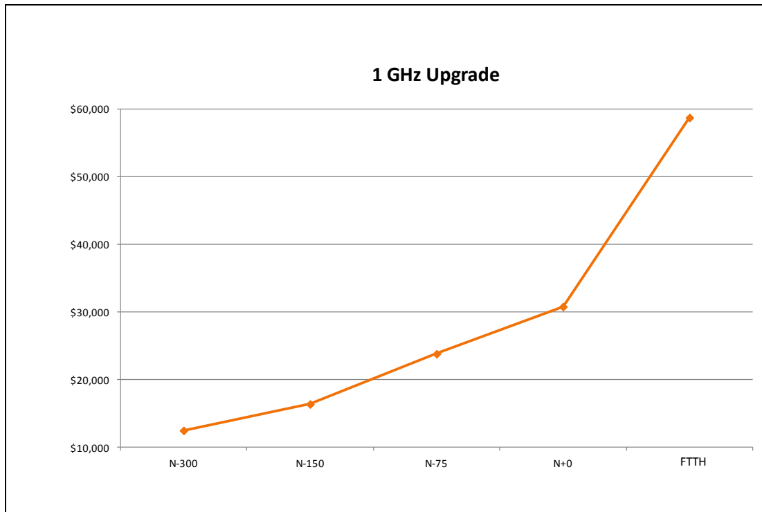
Figure 7 – Example 1 GHz/85 MHz Upgrade Costs vs. FTTP
