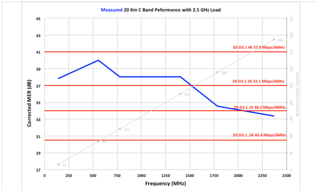
Figure 21 – HPON Downstream RF Performance
