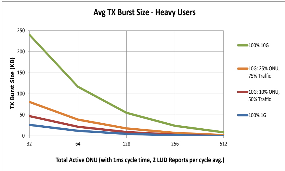
Figure 30 – Average TX Burst Size for Heavy Users
