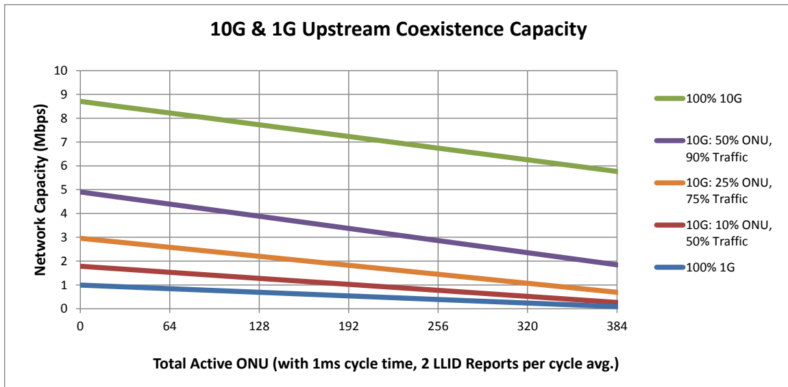
Figure 26 – 10G & 1G Upstream Coexistence Capacity
