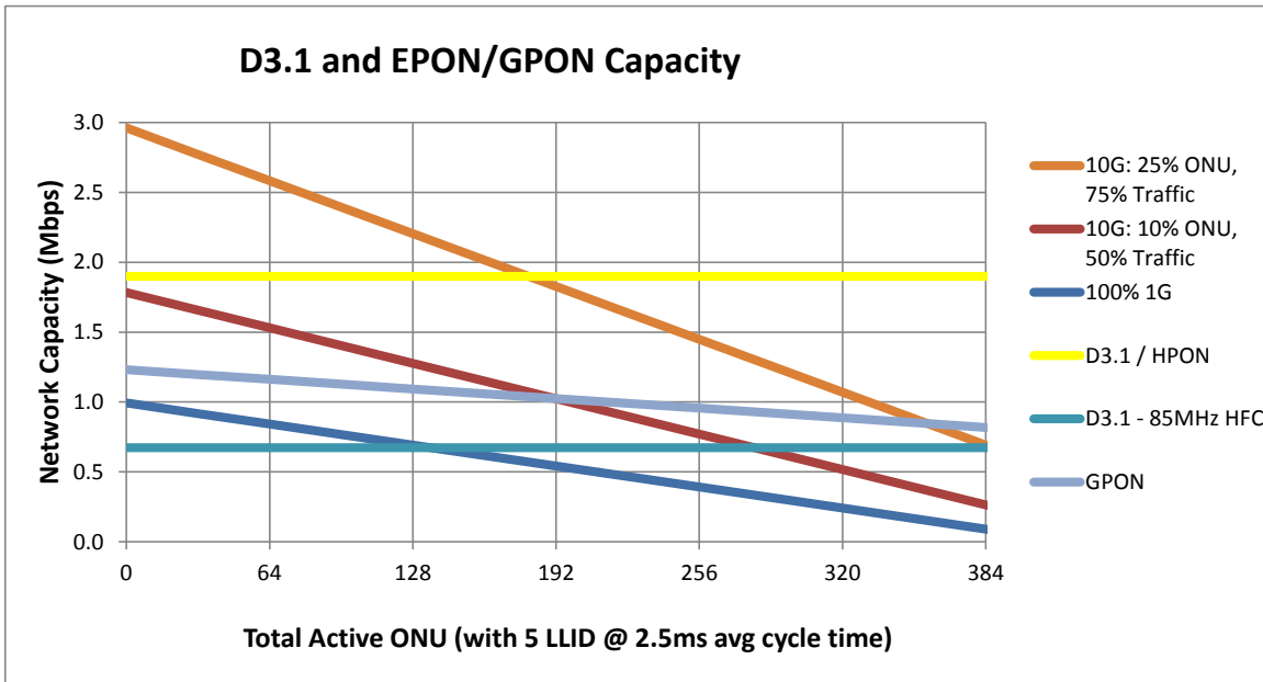
Figure 28 – D3.1 and EPON/GPON Capacity
