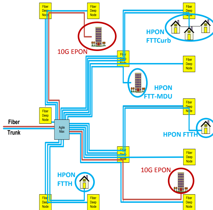
Figure 14 – HPON FTTP Migration: FTTP for More Performance Customers
