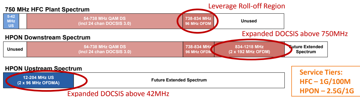
Figure 9 – HFC & HPON Spectrum Overlay
