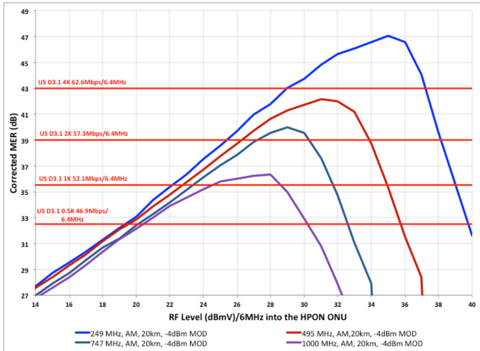
Figure 19 – HPON US MER for Various RF Spectrum
