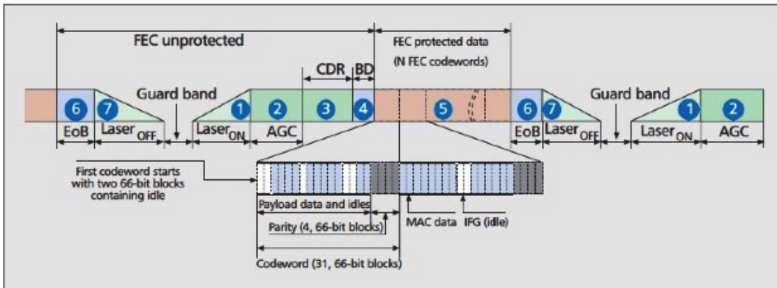
Figure 1. Internal structure of the upstream channel data burst in 10G-EPON.
