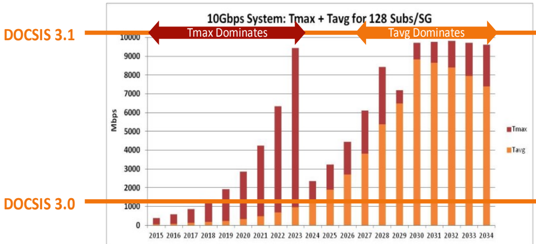
Figure 5 – Capacity Needs over Time, 128 Subs per SG
