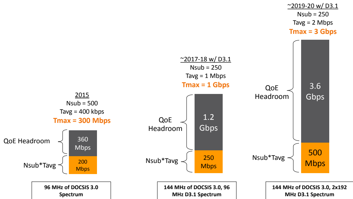
Figure 3 – Traffic Engineering with DOCSIS 3.1
