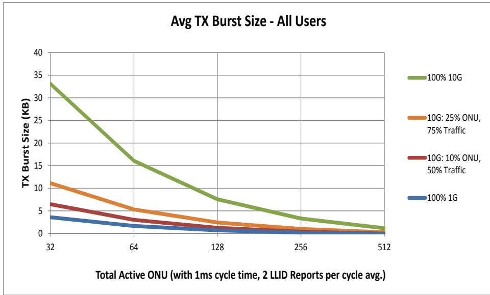
Figure 29 – Avg TX Burst Size, Traffic Evenly Distributed
