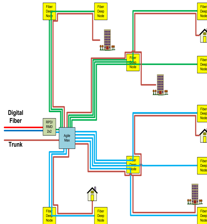
Figure 17 – HPON and Distributed Architecture: Shared Remote Device
