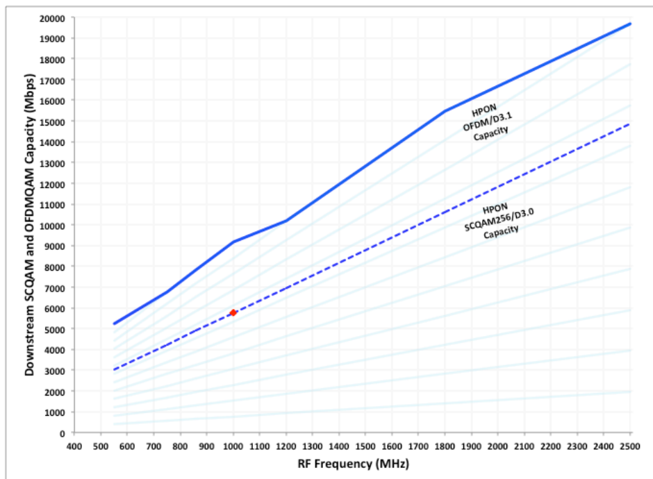
Figure 22 – HPON Downstream RF Capacity, OFDM v SC-QAM
