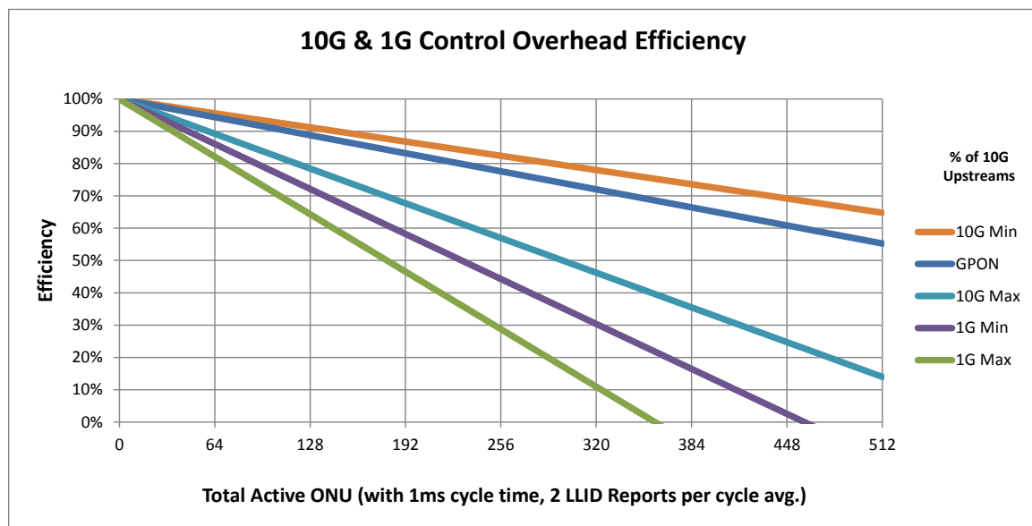
Figure 25 – 10G & 1G Control Overhead Efficiency
