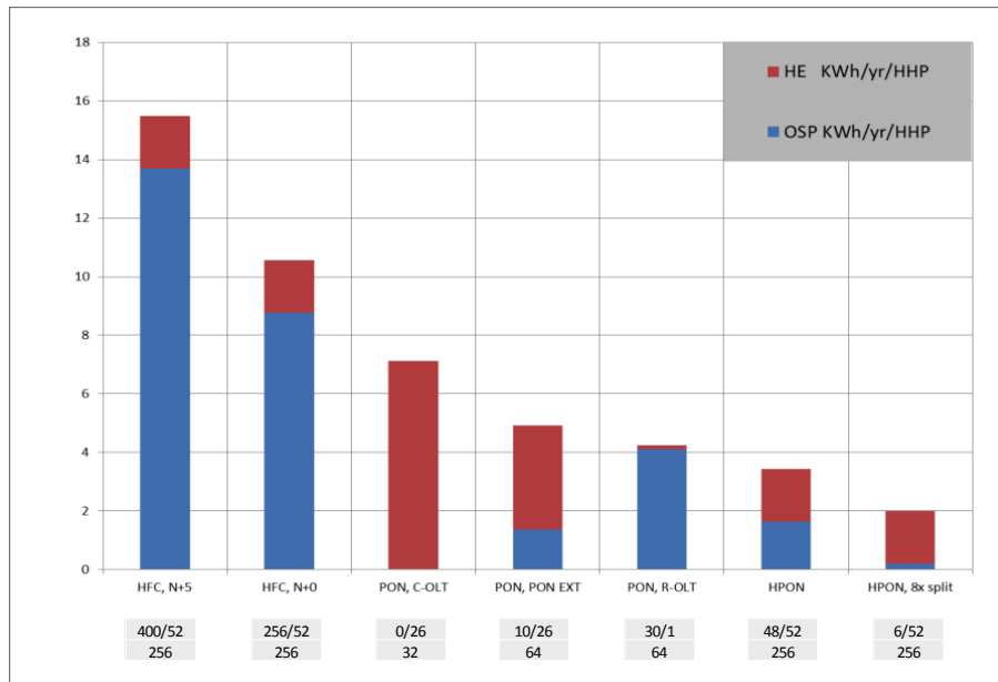
Figure 33 – Relative Energy Costs for HFC, EPON and HPON Systems
