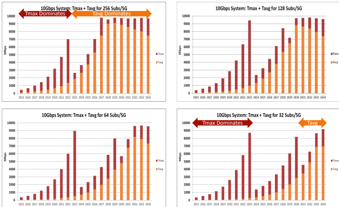
Figure 6 – Capacity Needs over Time, Various SG sizes
