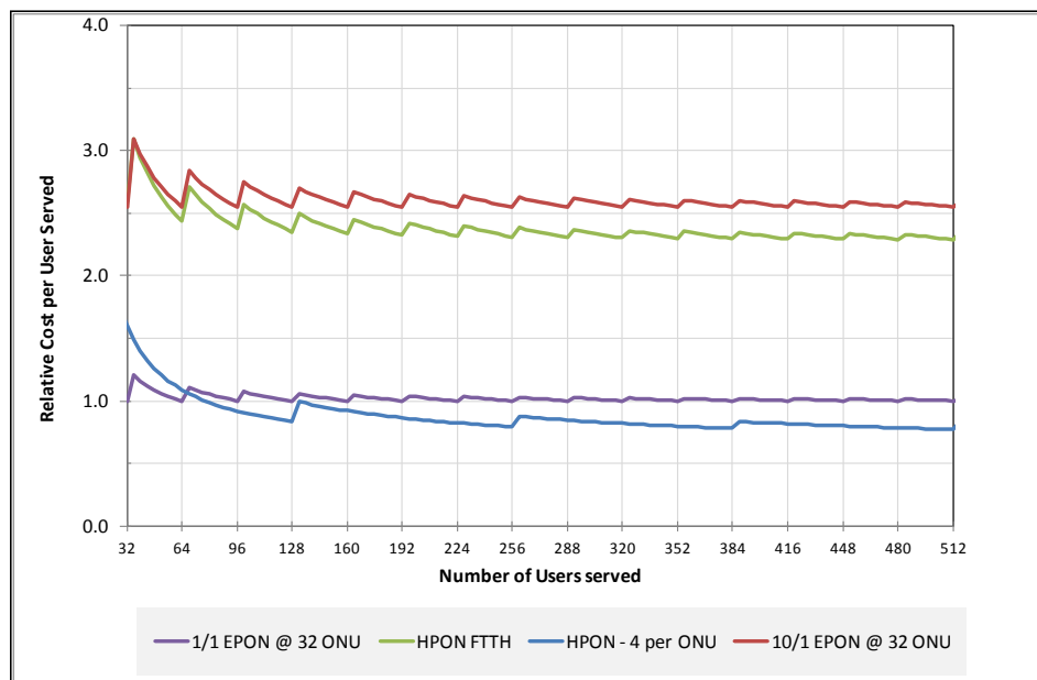
Figure 31 – Relative Costs for EPON & HPON Systems
