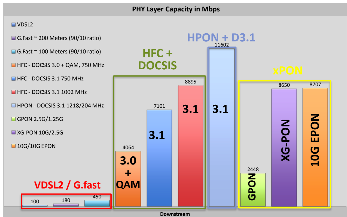
Figure 10 – Downstream Capacity: HFC & HPON vs. xPON
