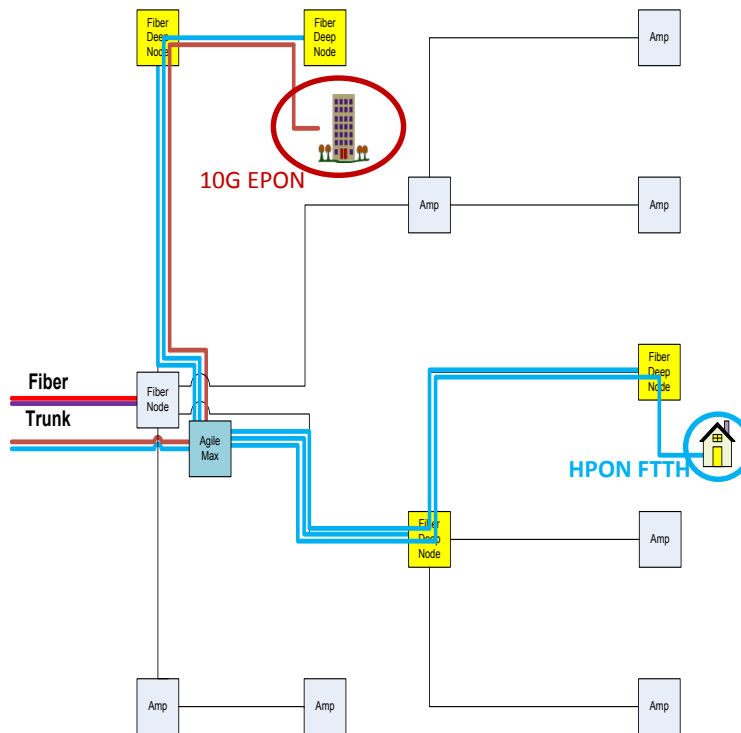
Figure 13 – HPON FTTP Migration: FTTP for Select Top Customers
