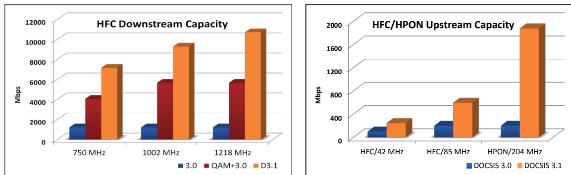
Figure 8- HFC Upstream and Downstream Capacity
