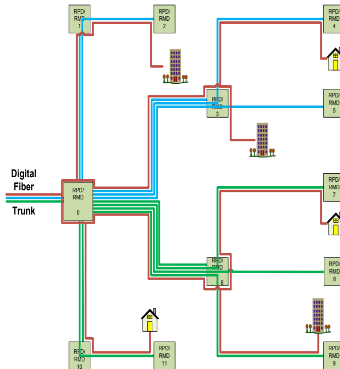
Figure 16 – Distributed Architecture: Conventional Wisdom
