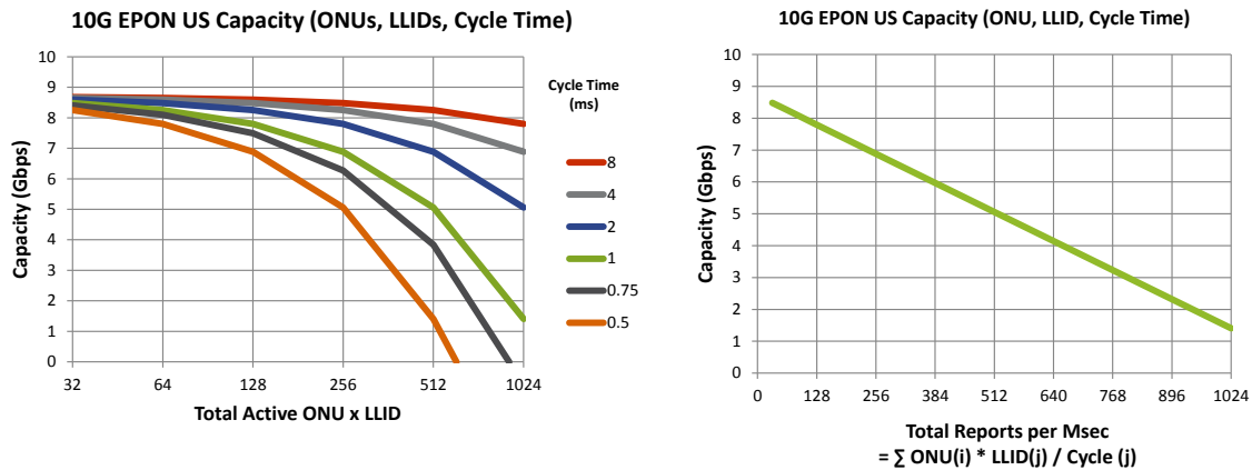
Figure 24 – 10G EPON Upstream Cycle Time & ONU Impacts
