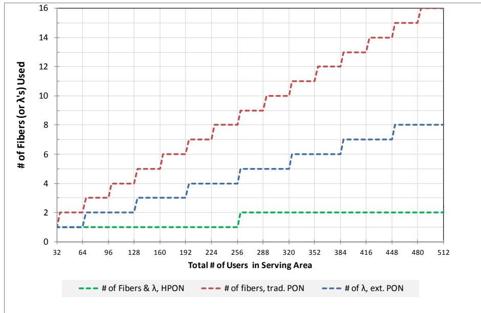
Figure 32 – Fiber Trunks, Wavelengths and OLT/CCAP Ports Required
