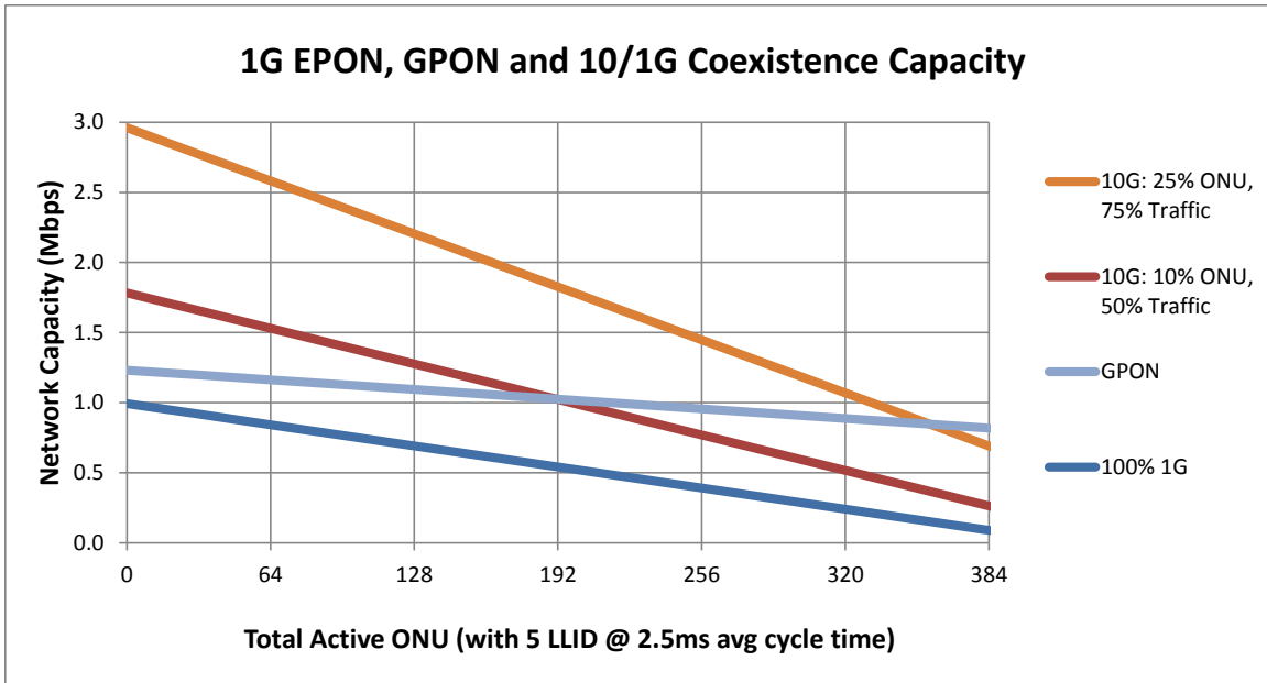
Figure 27 – 1G EPON, 10/10 & 10/1 Coexistence, and GPON
