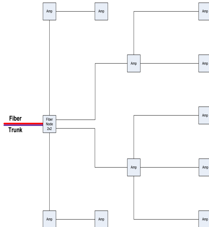
Figure 12 – HPON FTTP Migration: Baseline
