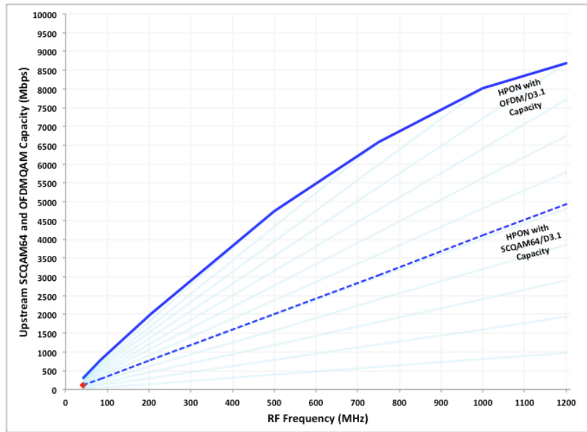
Figure 20 – HPON US Capacity – OFDMA vs. SC-QAM
