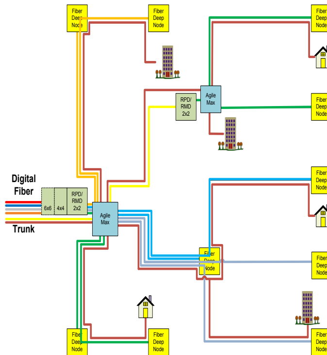
Figure 18 – HPON and Distributed Architecture: SG Segmentation as needed
