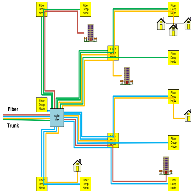
Figure 15 – HPON FTTP Migration: SG Segmentation as Needed
